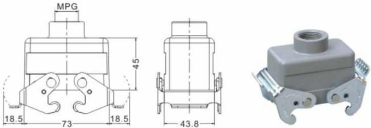
Right socket for hood: CMB_10_Fx_DF_010
