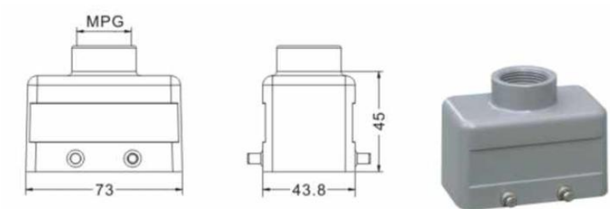
Curved socket: CMB_10_Fx_D_010
