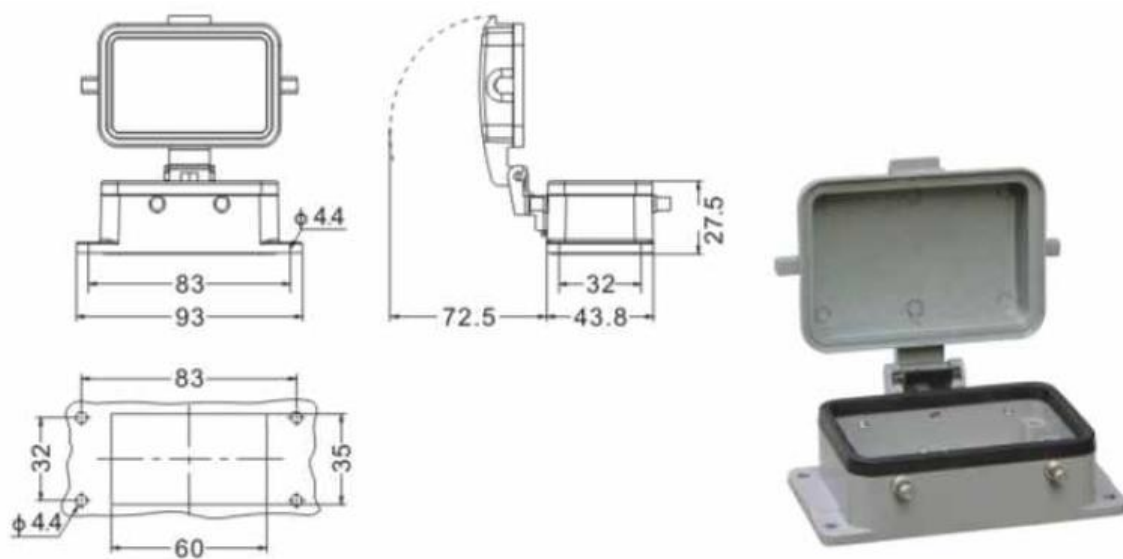
Plug with hood, to be fixed: CMB_10_Px_DF_010
