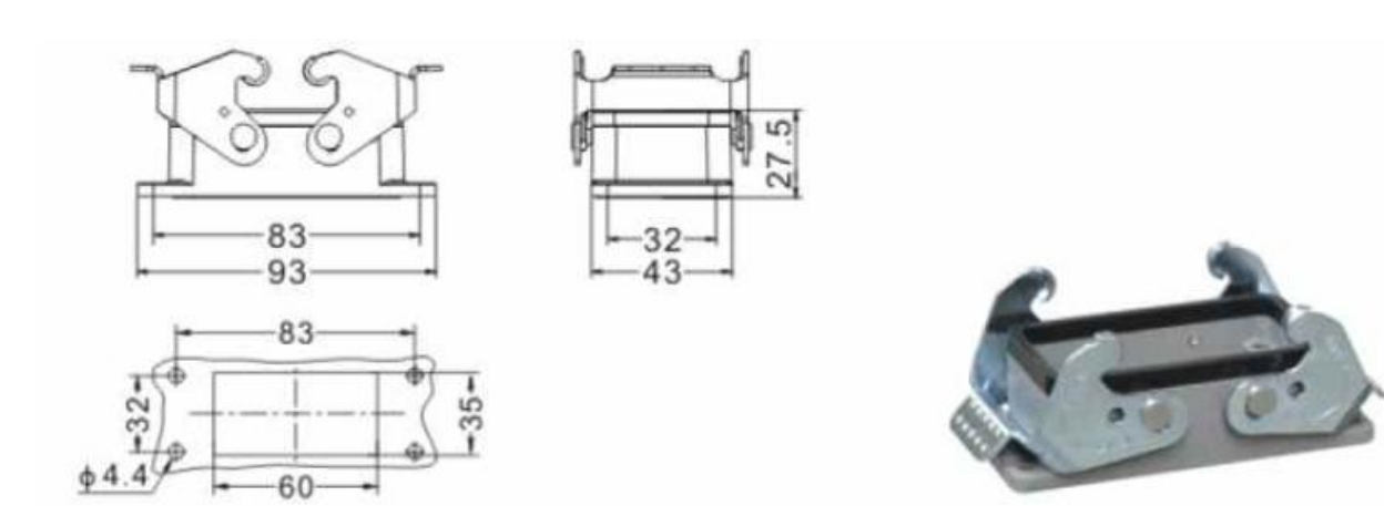
Plug with base to be fixed on the electrical box: CMB_10_Px_D_010
