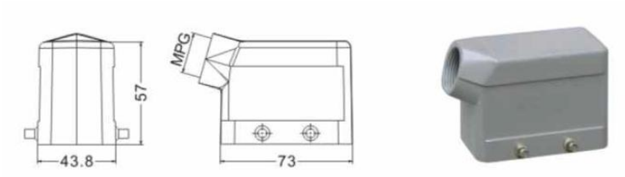
Curved socket: CMB_10_Fx_L_010
